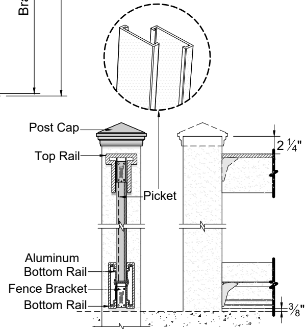
CUT VIEWS
